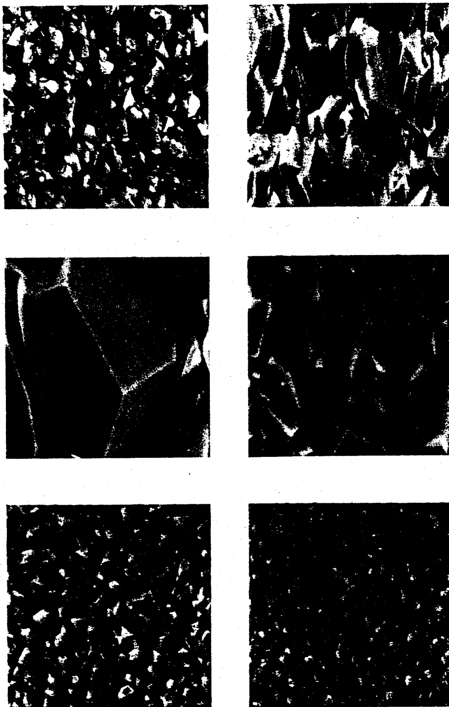
FIGURE 2. 24\ \mu\text{m} \times 24\ \mu\text{m} SEM images of In-doped CdTe films at different temperature. CdTe source and substrata temperature used for all samples are 600\ ^\circ\text{C} and 500\ ^\circ\text{C} respectively. Indium source temperature in images are: a) 560\ ^\circ\text{C} , b) 600\ ^\circ\text{C} , c) 640\ ^\circ\text{C} , d) 650\ ^\circ\text{C} , e) 670\ ^\circ\text{C} and f) 720\ ^\circ\text{C} . Serial RC1.
