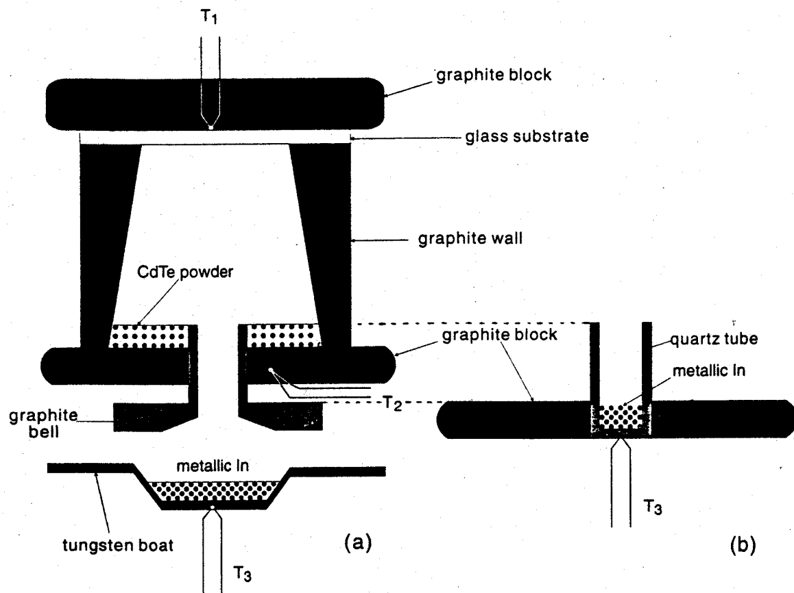
FIGURE 1. Artist's rendition of the chamber used for CSVT combined with free evaporation: a) CSVT-FE with external indium source, b) CSVT-FE with internal indium source.
